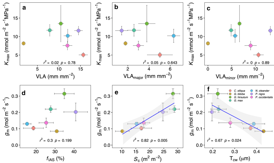
Fig. 3 Impacts of leaf anatomical traits on mesophyll conductance ( g_m ) and maximum leaf hydraulic conductance ( K_{max} ). VLA, Leaf vein density; VLA major , major vein density; VLA minor , minor vein density; f_{IAS} , fraction of leaf mesophyll volume occupied by intercellular air space; S_c , total chloroplast surface area exposed to intercellular air space per unit of leaf surface area; and T_{cw} , cell wall thickness
