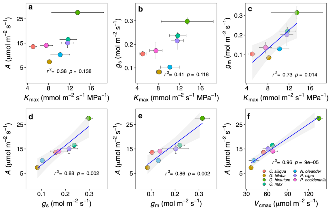
Fig. 2 Correlations among efficiency traits. The correlation between traits was fitted using the linear model, and the shade areas around lines indicate the 95% of confidence intervals. A , light-saturated pho-
